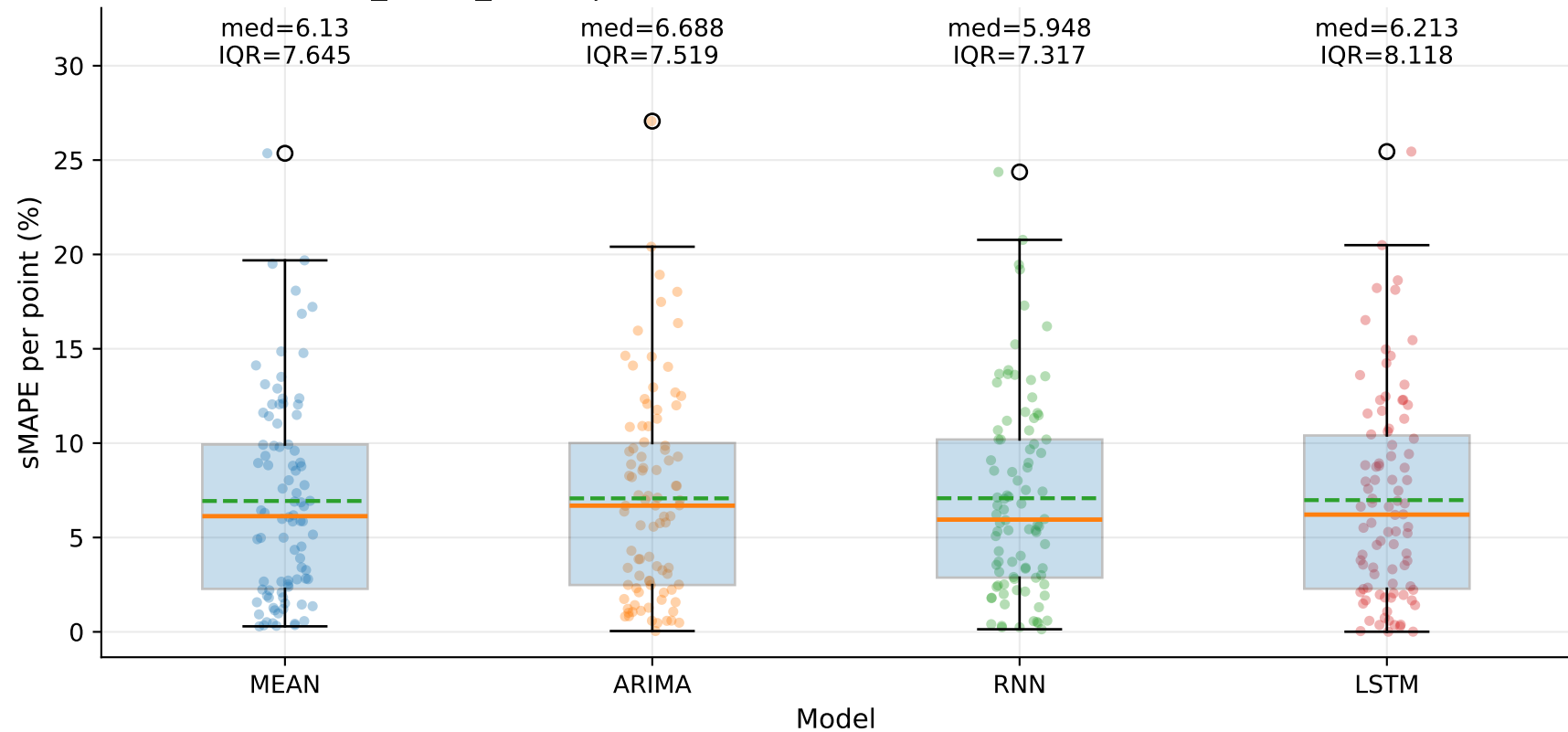
M5_YHUR_SHUR | sMAPE distribution by model — TSEC (step=1)
