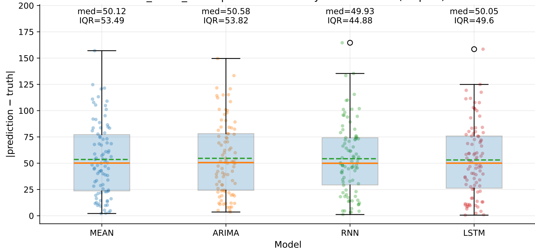
M5_YHUR_SHUR | Absolute error by model — TSE (step=1)
