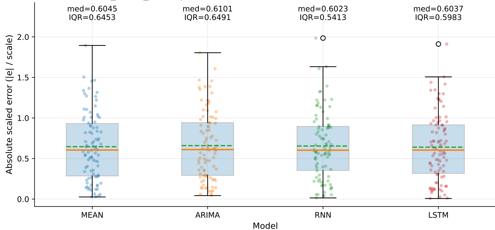
M5_YHUR_SHUR | MASE-point distribution by model — TSE (step=1)
