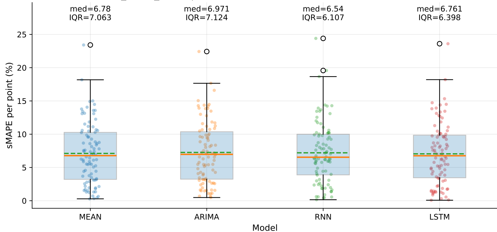
M5_YHUR_SHUR | sMAPE distribution by model — TSE (step=1)
