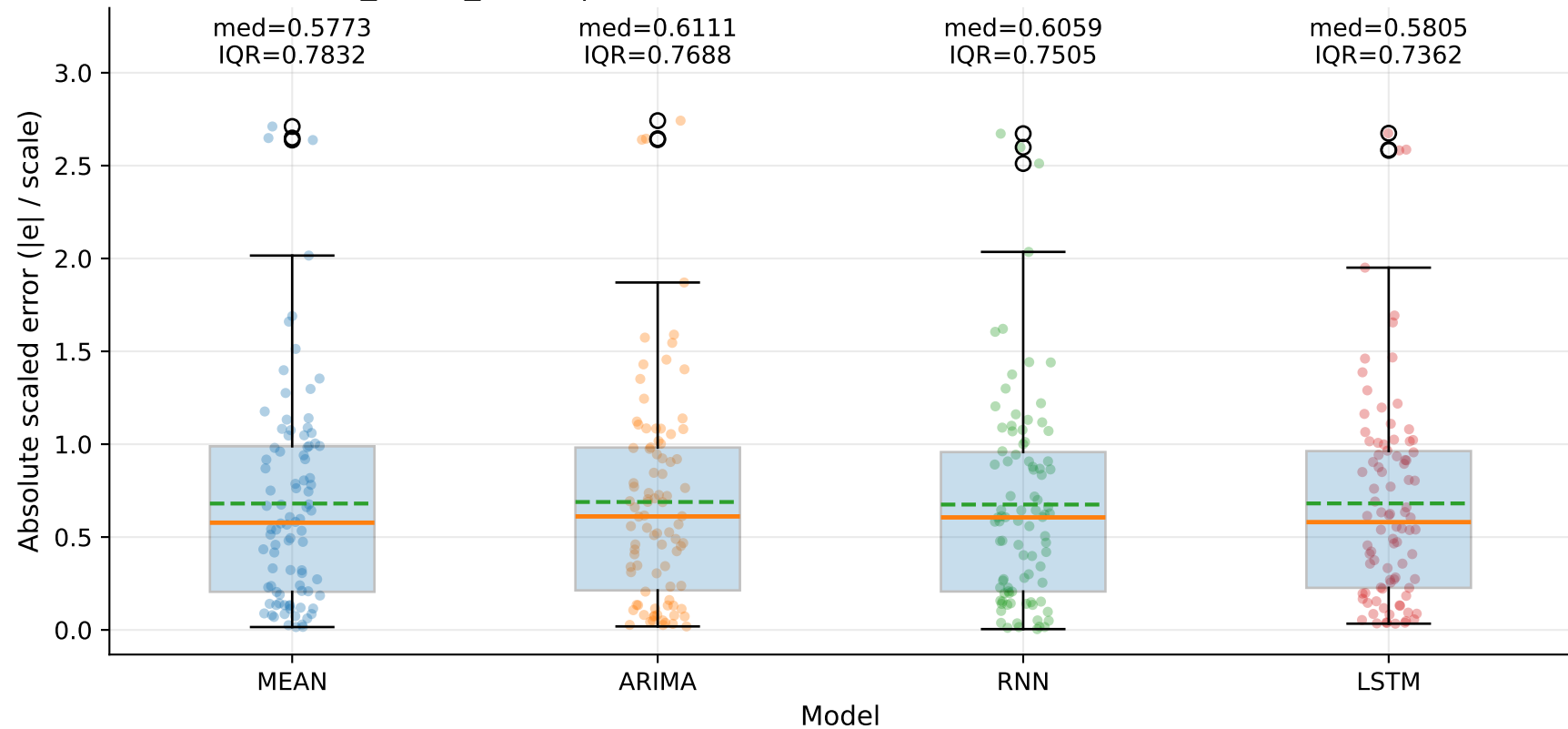
M5_YHUR_SHUR | MASE-point distribution by model — Yd (step=1)
