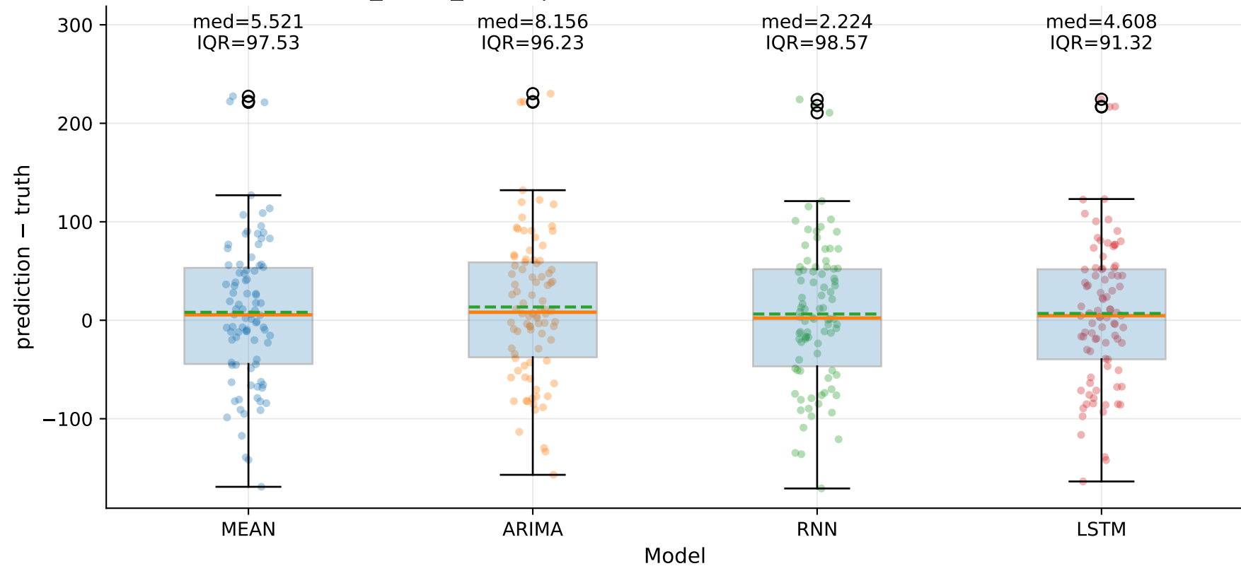
M5_YHUR_SHUR | Signed error by model — Yd (step=1)
