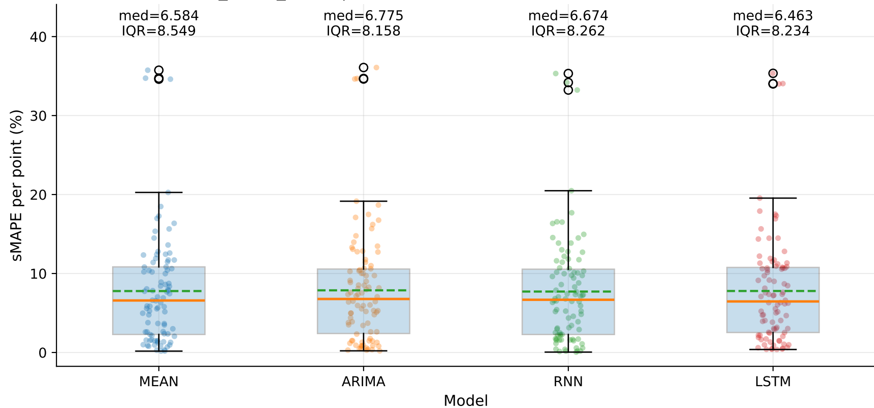
M5_YHUR_SHUR | sMAPE distribution by model — Yd (step=1)
