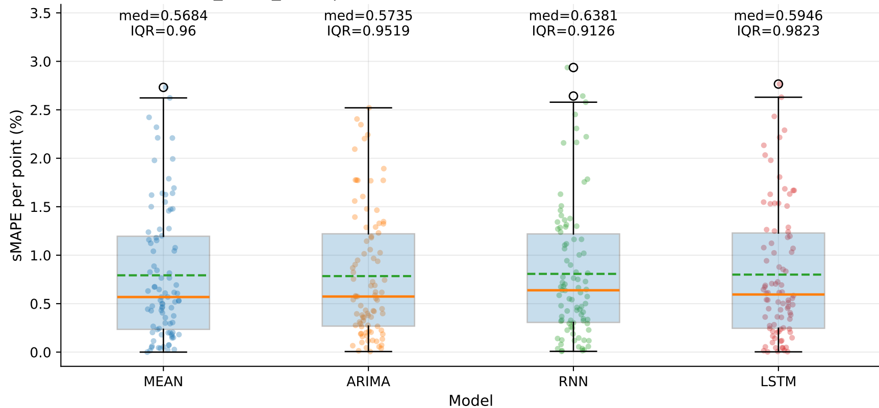
M5_YHUR_SLUR | sMAPE distribution by model — TSEC (step=1)
