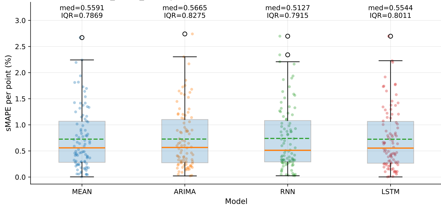
M5_YHUR_SLUR | sMAPE distribution by model — TSE (step=1)
