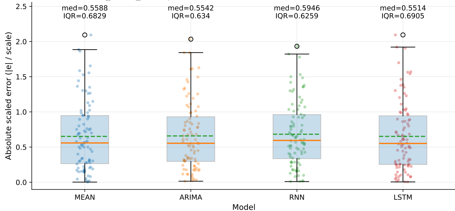
M5_YHUR_SLUR | MASE-point distribution by model — Yd (step=1)
