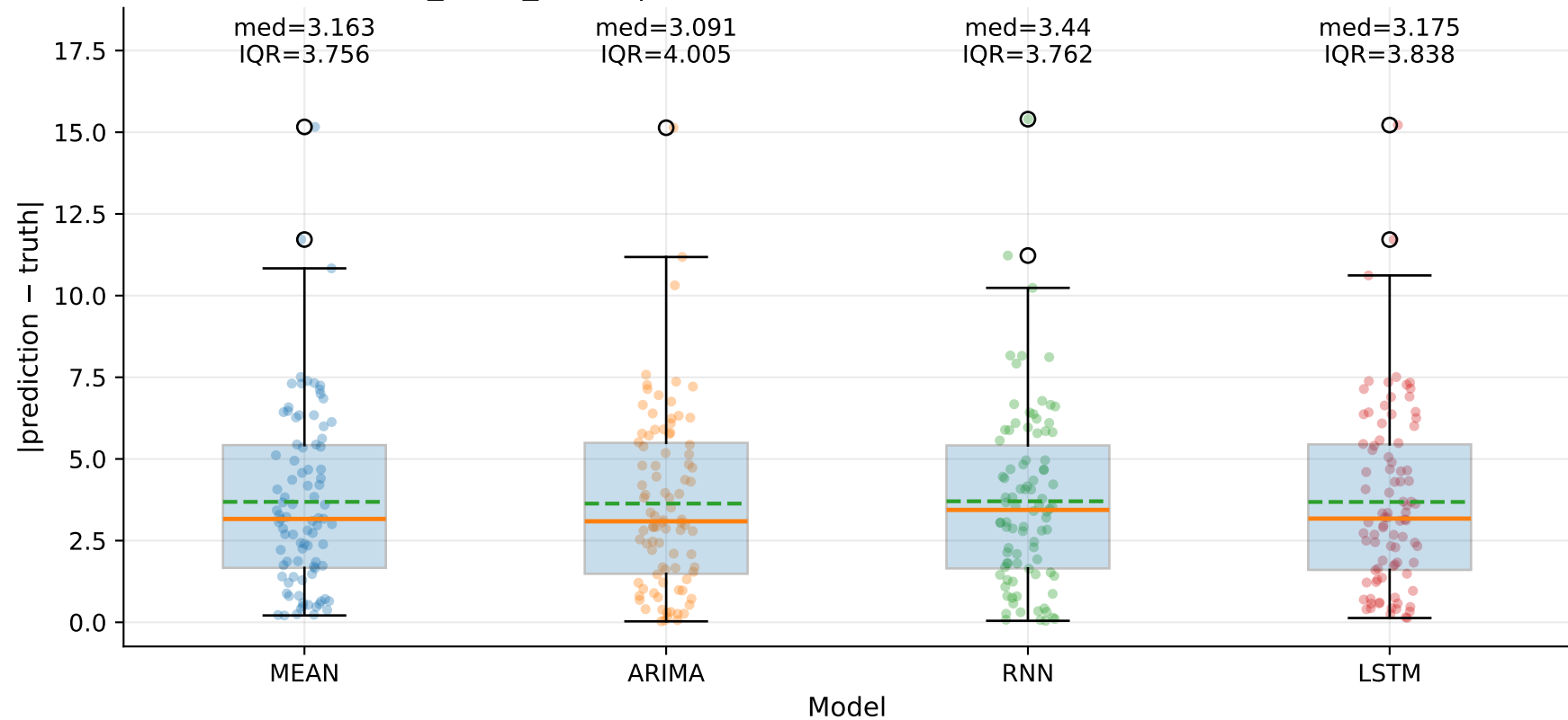
M5_YLUR_SHUR | Absolute error by model — TSEC (step=1)
