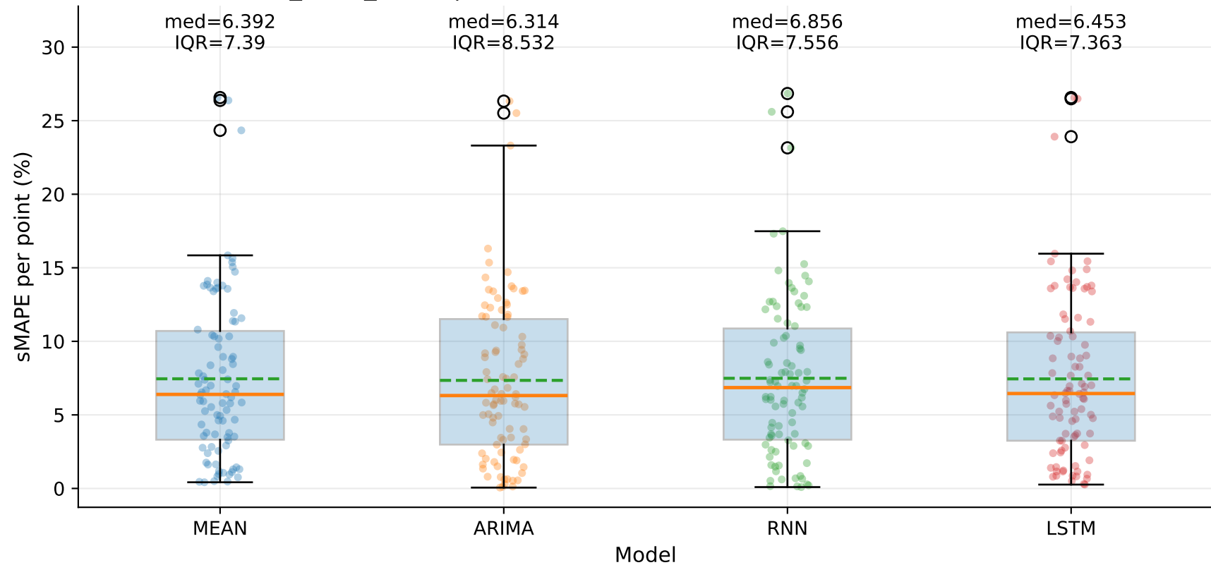
M5_YLUR_SHUR | sMAPE distribution by model — TSEC (step=1)
