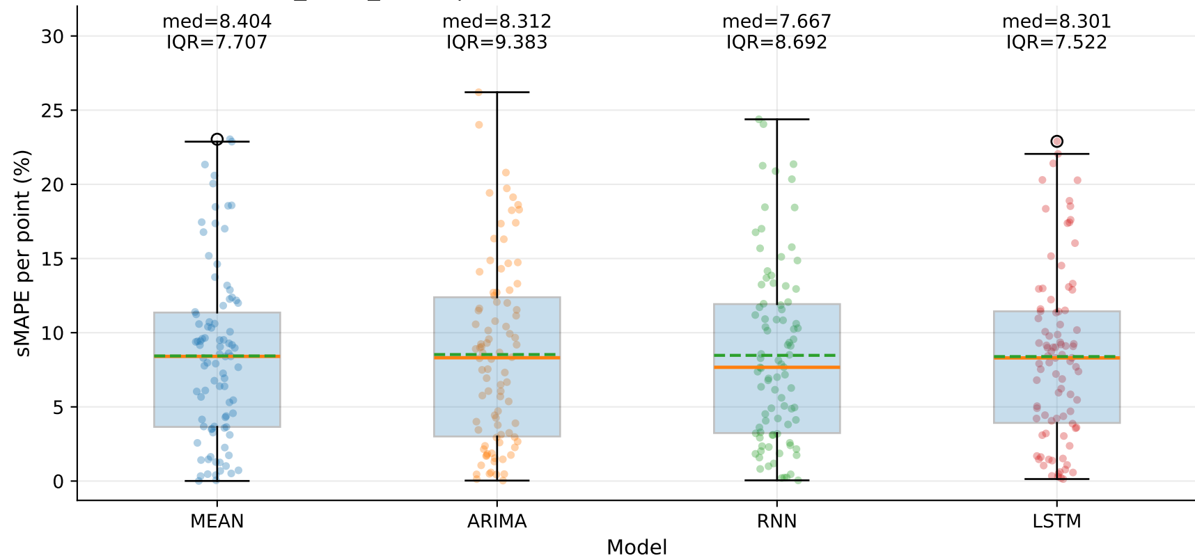
M5_YLUR_SHUR | sMAPE distribution by model — TSE (step=1)
