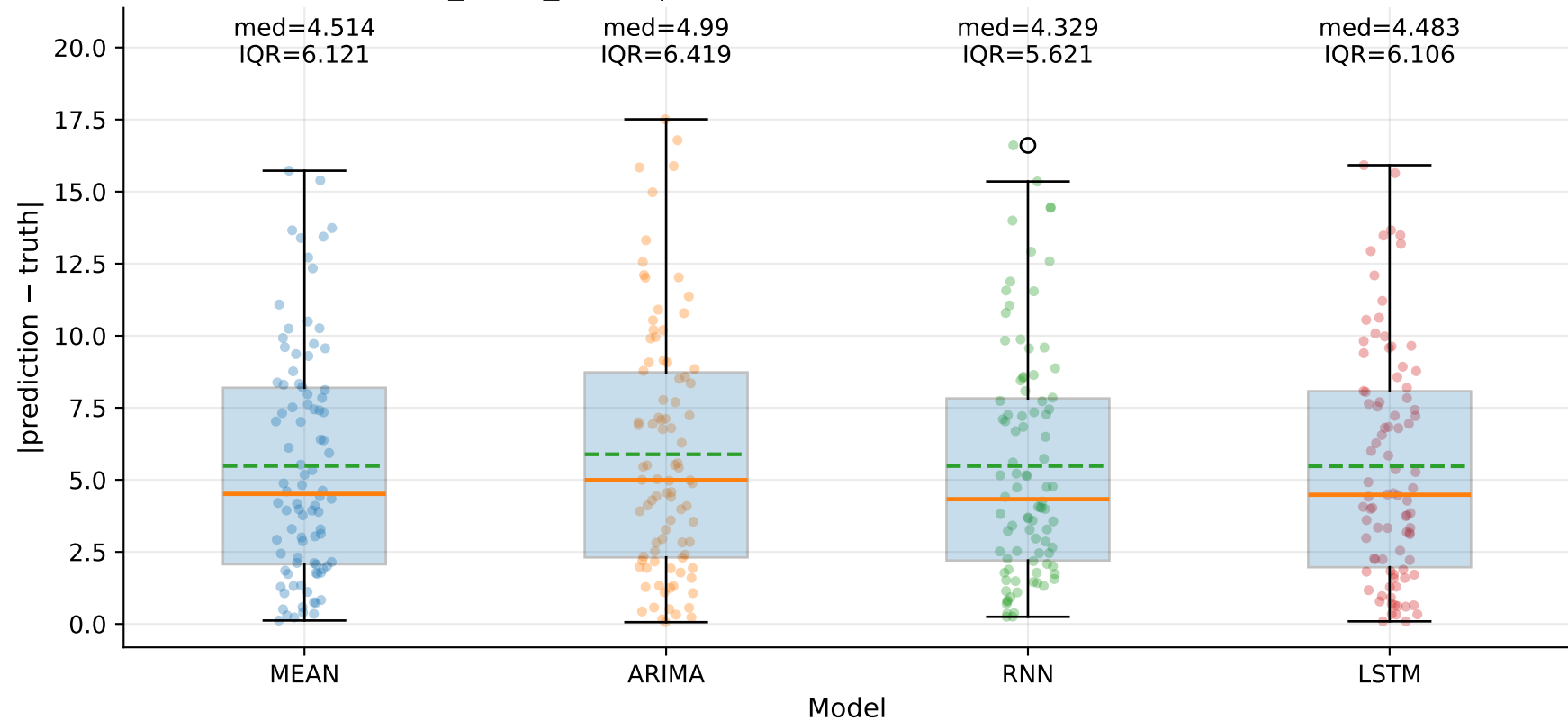
M5_YLUR_SHUR | Absolute error by model — Yd (step=1)
