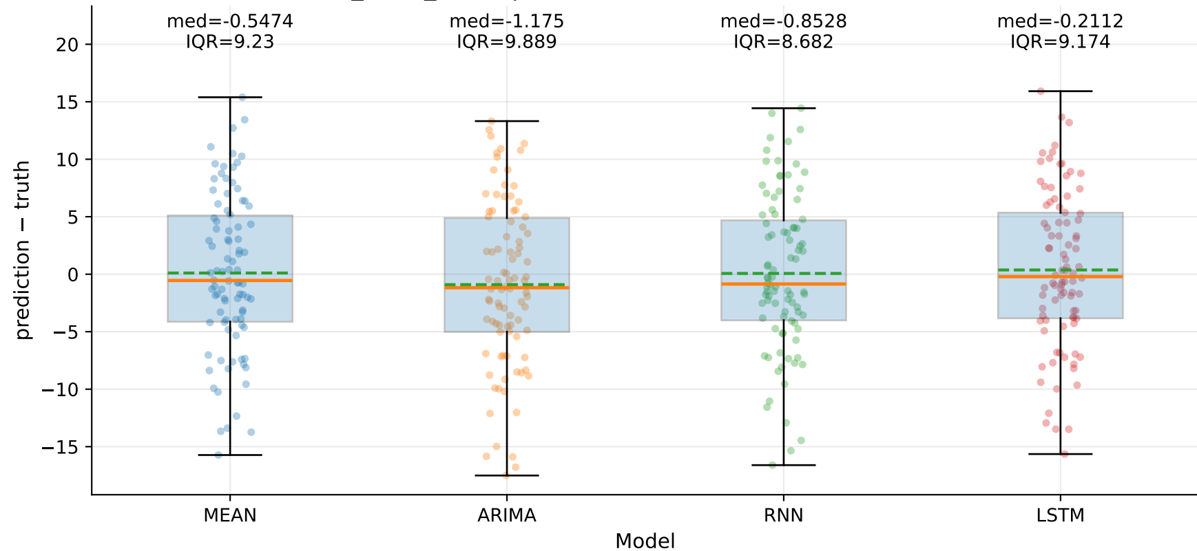
M5_YLUR_SHUR | Signed error by model — Yd (step=1)
