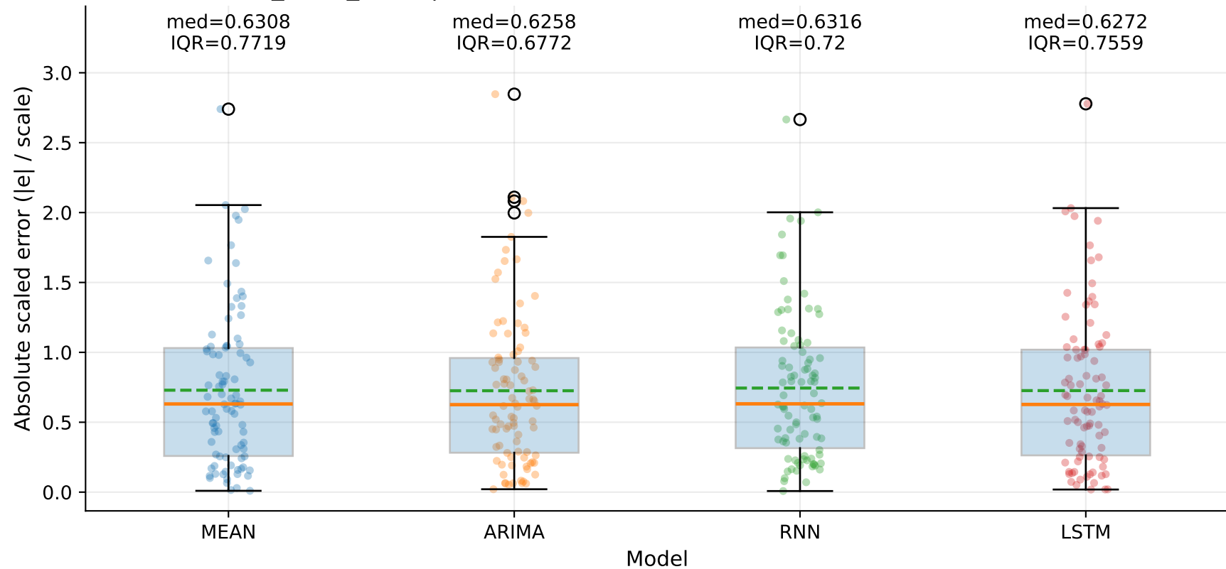
M5_YLUR_SLUR | MASE-point distribution by model — TSEC (step=1)
