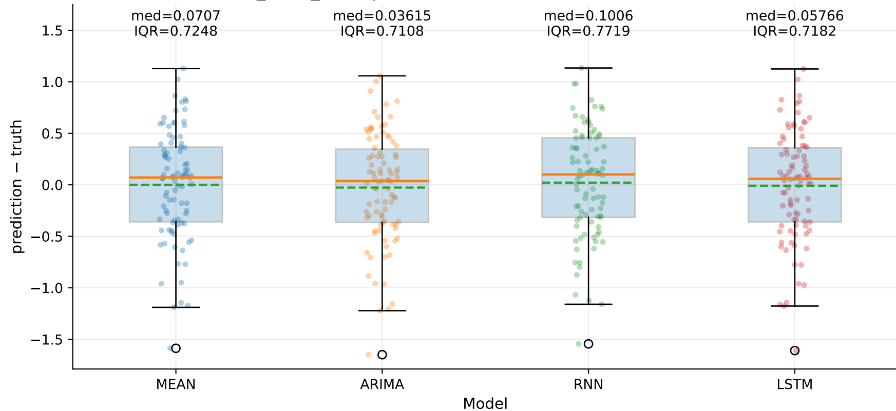
M5_YLUR_SLUR | Signed error by model — TSEC (step=1)
