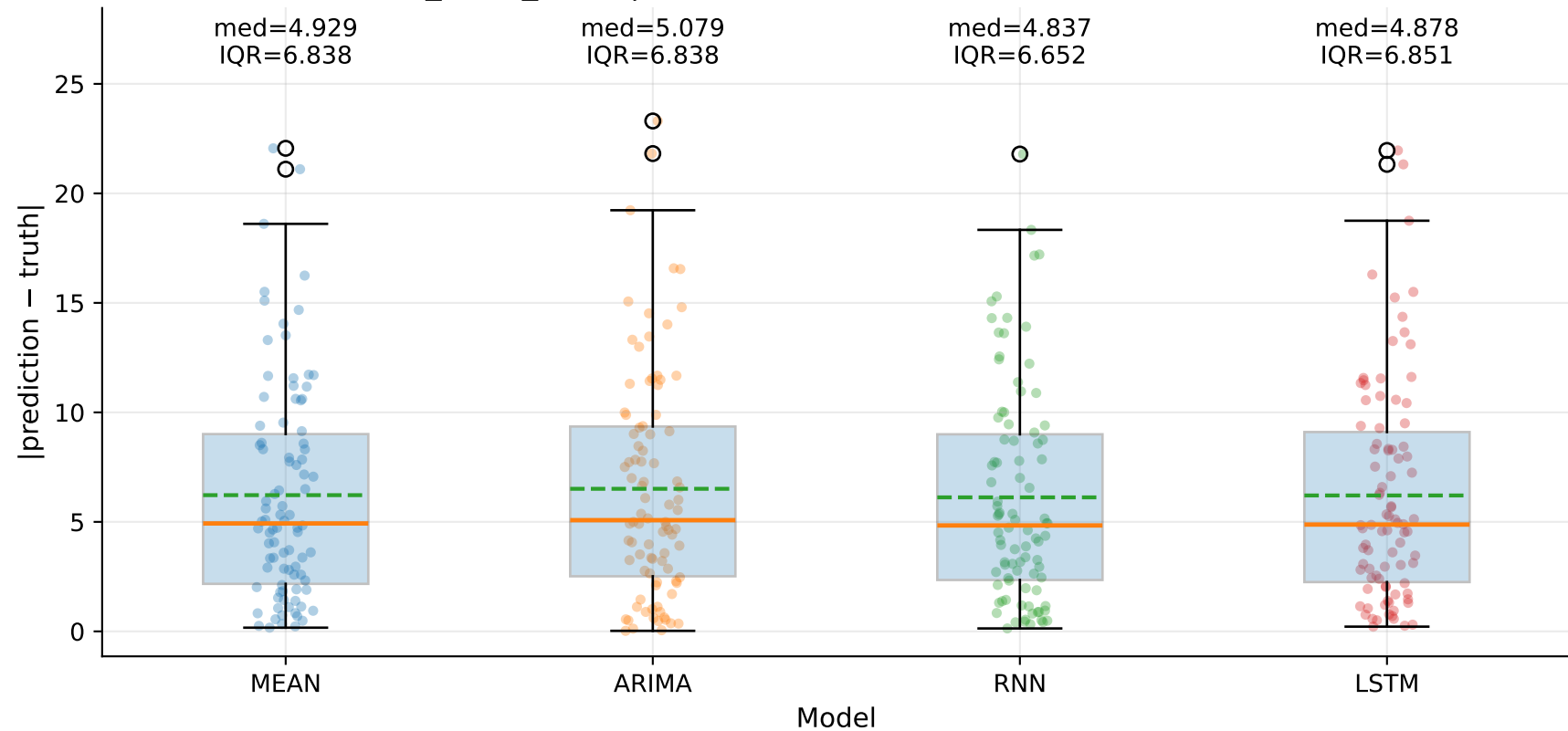
M5_YLUR_SLUR | Absolute error by model — TSE (step=1)
