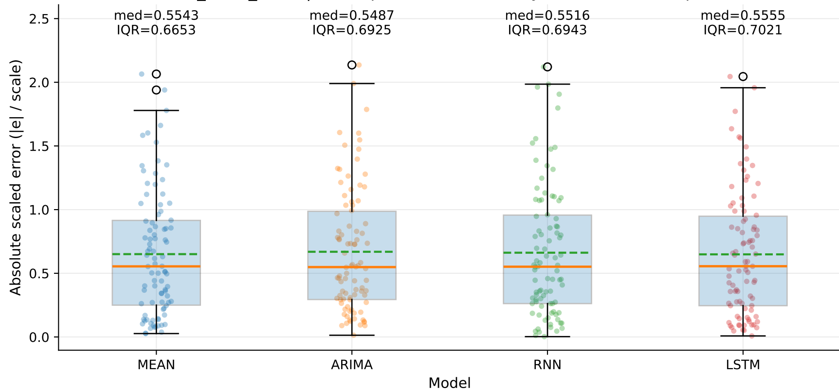
M5_YLUR_SLUR | MASE-point distribution by model — Yd (step=1)
