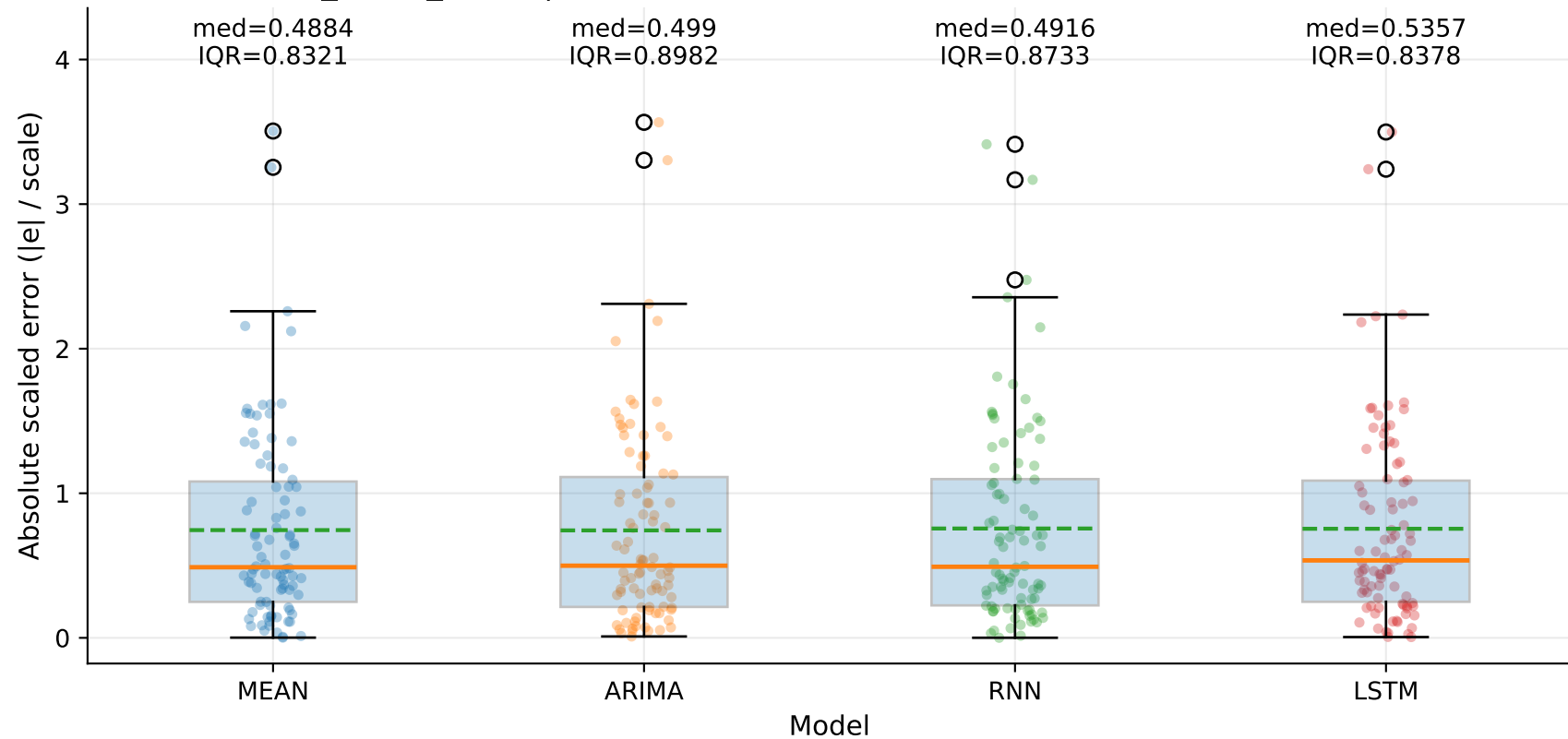
M6_YHUR_SHUR | MASE-point distribution by model — TSEC (step=1)
