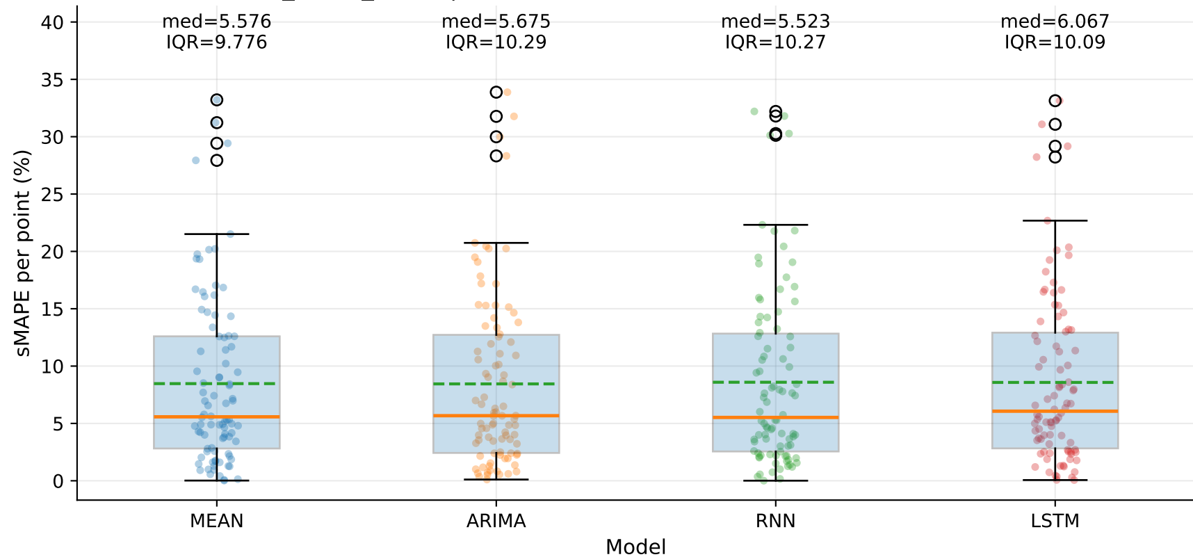
M6_YHUR_SHUR | sMAPE distribution by model — TSEC (step=1)
