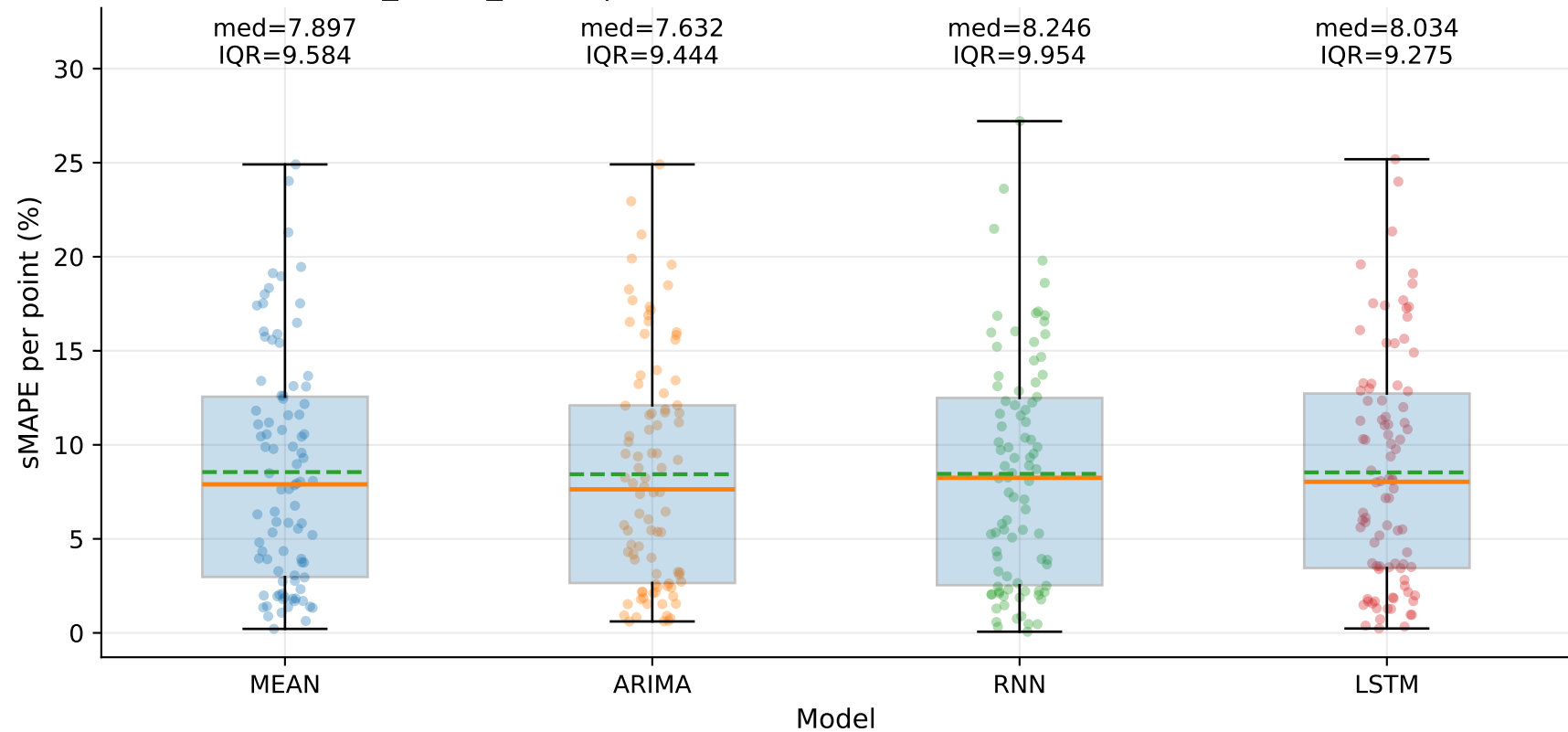
M6_YHUR_SHUR | sMAPE distribution by model — TSE (step=1)
