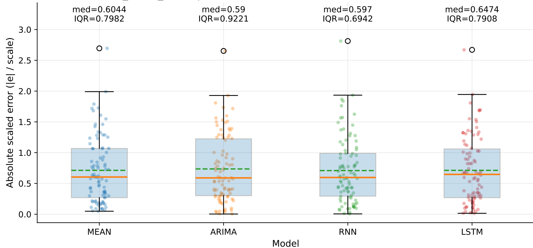
M6_YHUR_SHUR | MASE-point distribution by model — Yd (step=1)
