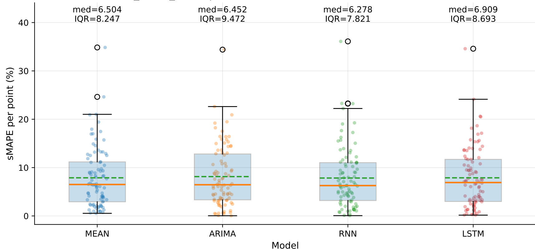
M6_YHUR_SHUR | sMAPE distribution by model — Yd (step=1)
