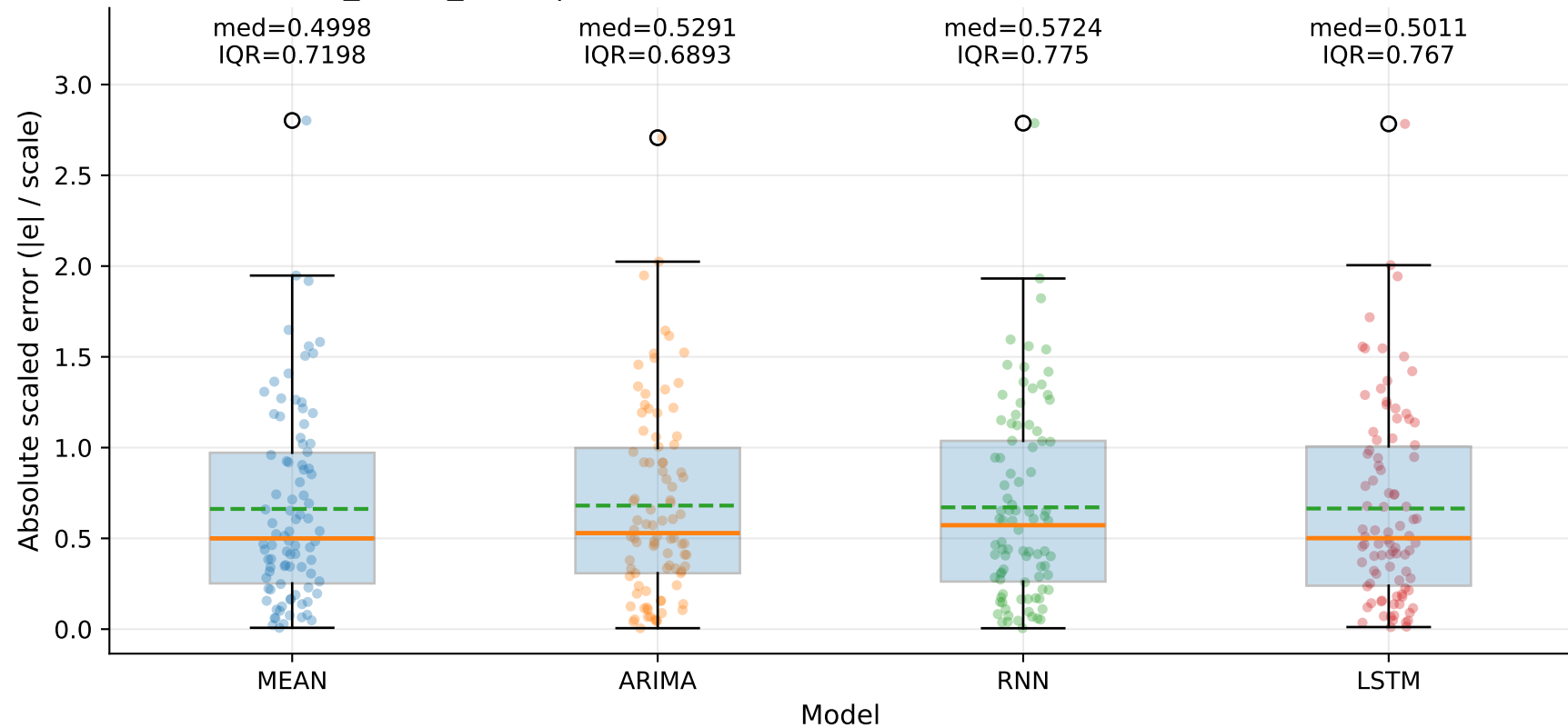
M6_YHUR_SLUR | MASE-point distribution by model — TSEC (step=1)
