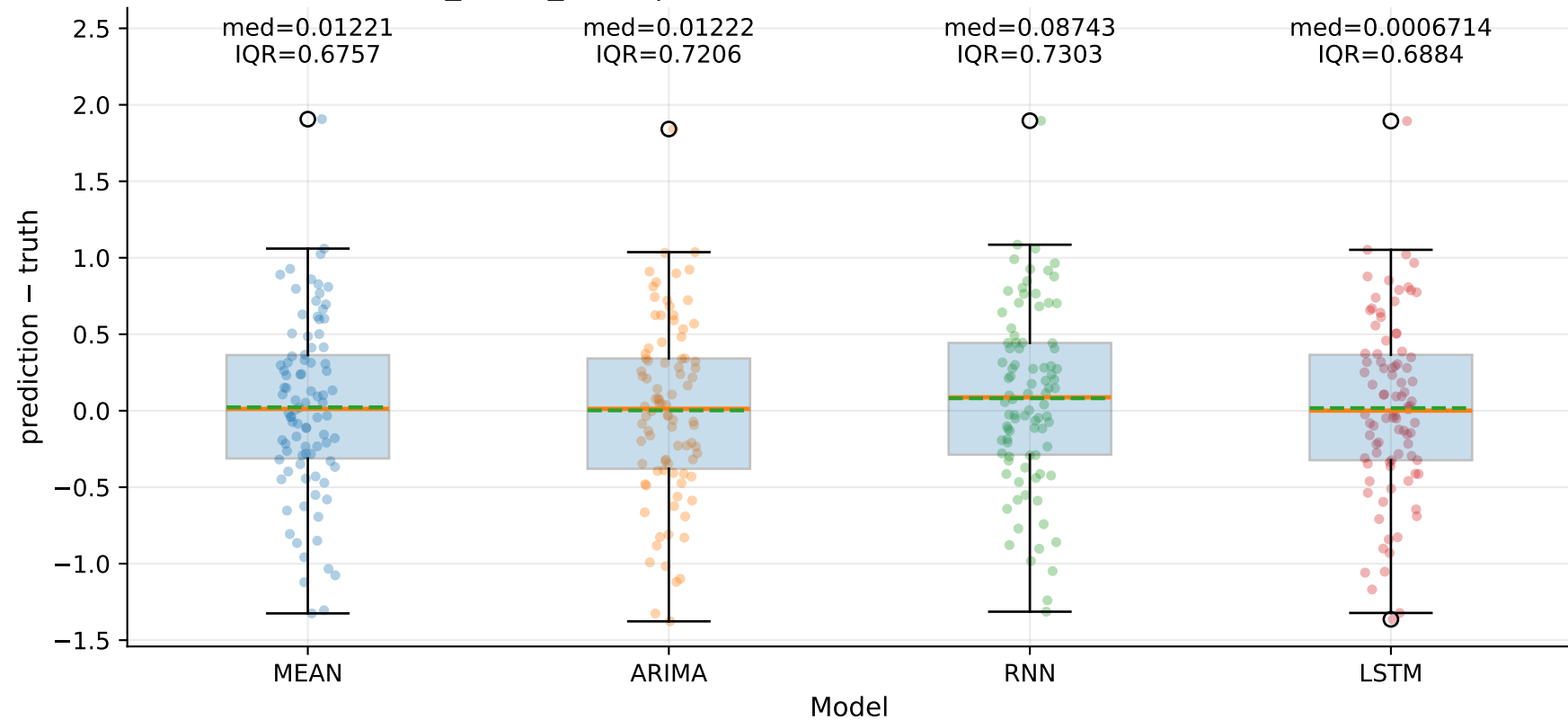
M6_YHUR_SLUR | Signed error by model — TSEC (step=1)
