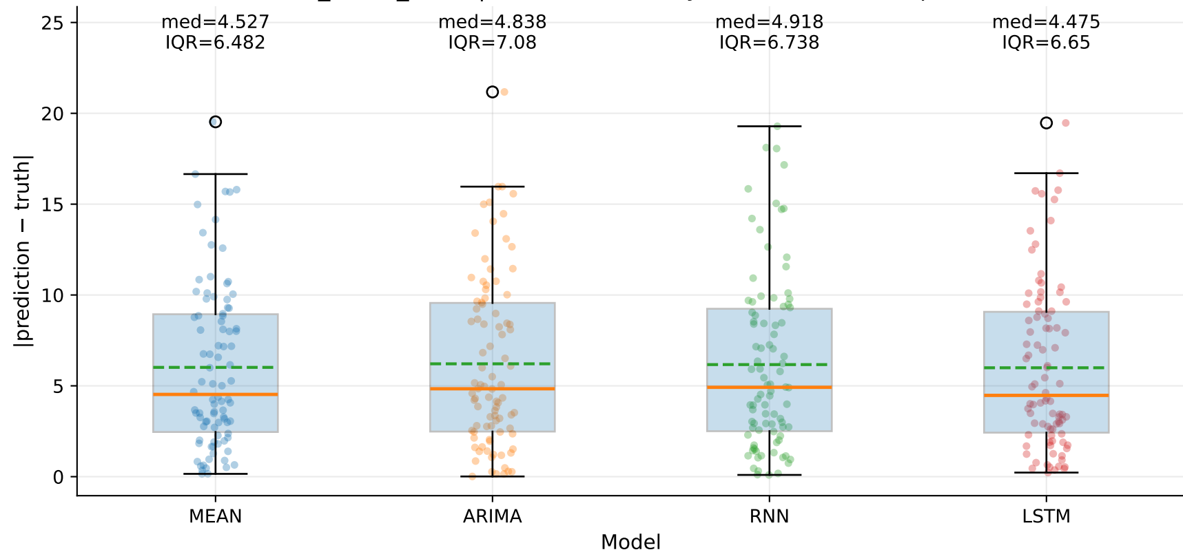
M6_YHUR_SLUR | Absolute error by model — TSE (step=1)
