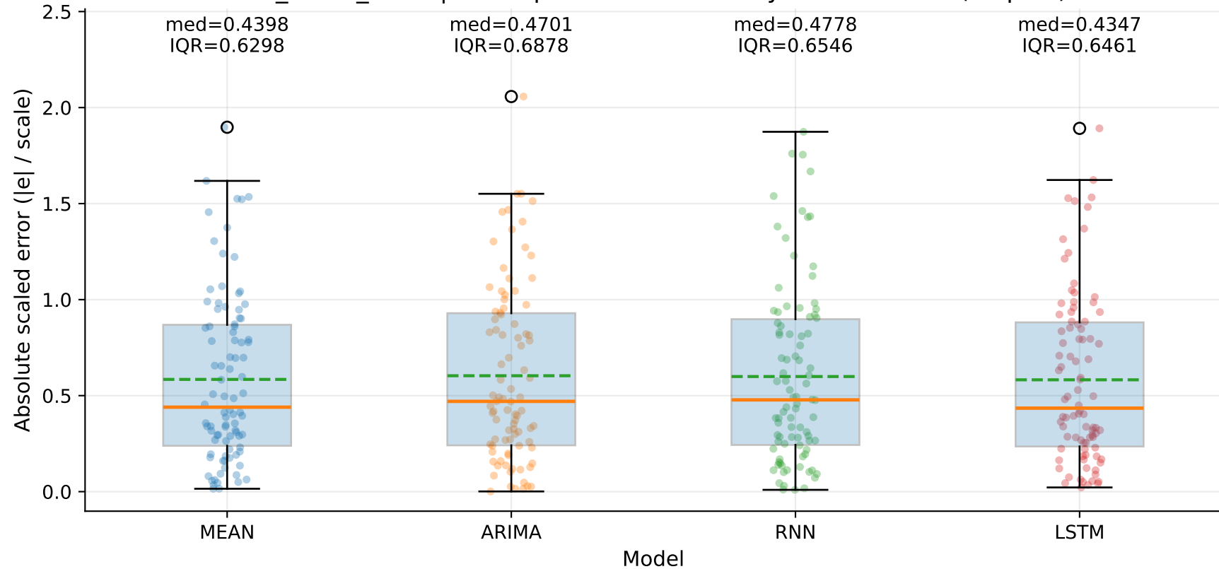
M6_YHUR_SLUR | MASE-point distribution by model — TSE (step=1)
