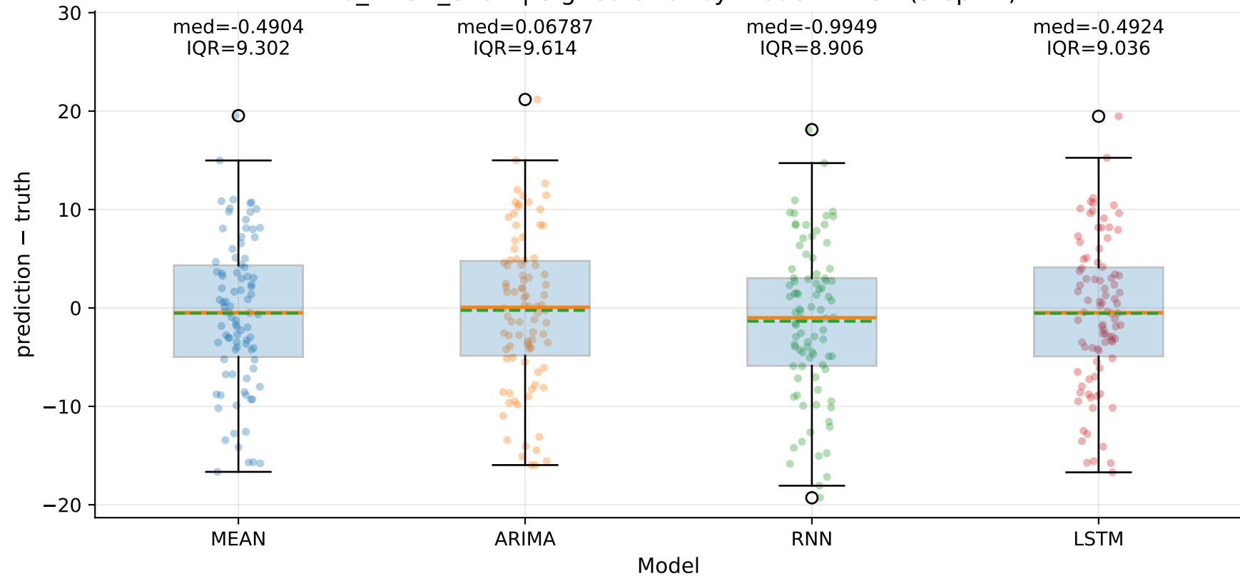
M6_YHUR_SLUR | Signed error by model — TSE (step=1)
