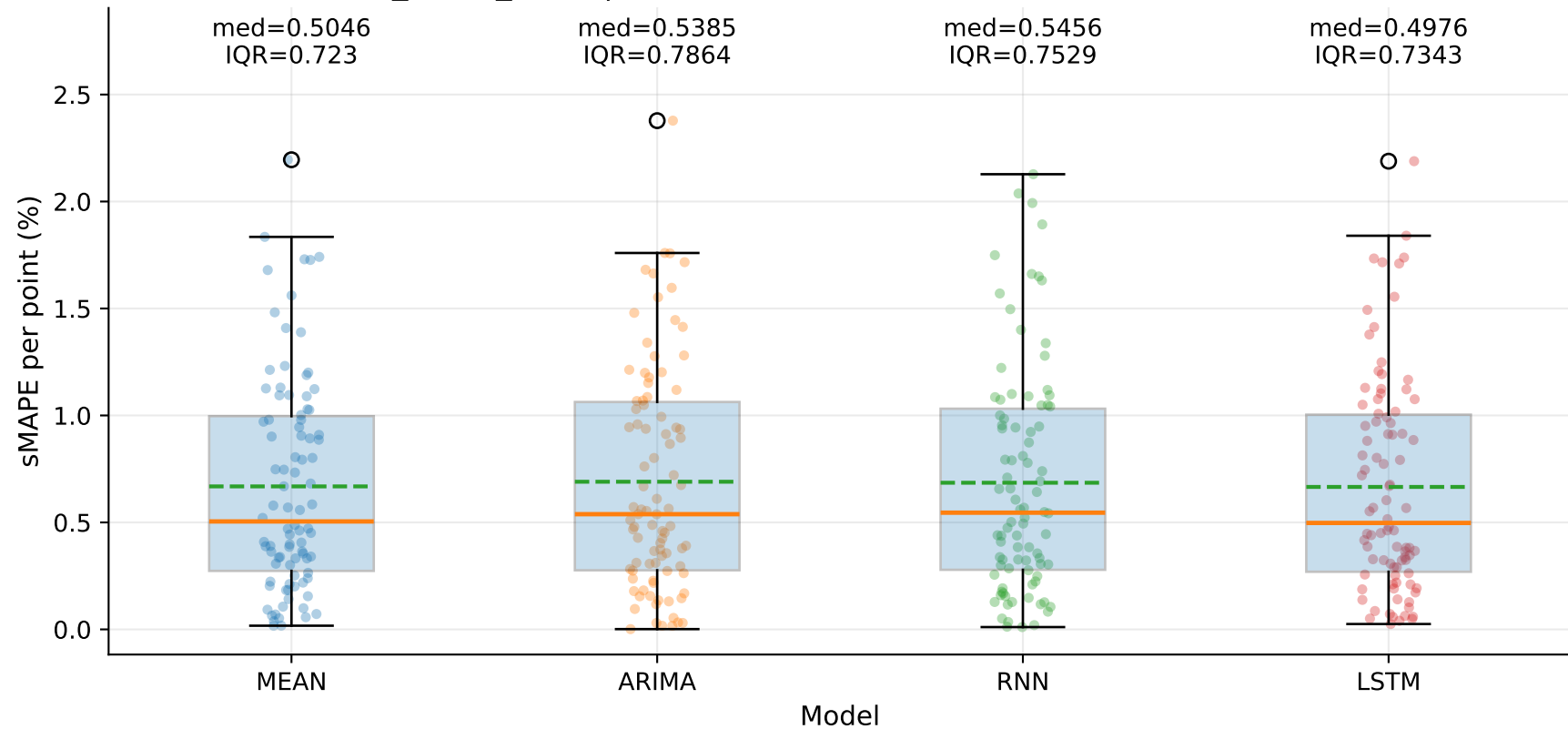
M6_YHUR_SLUR | sMAPE distribution by model — TSE (step=1)
