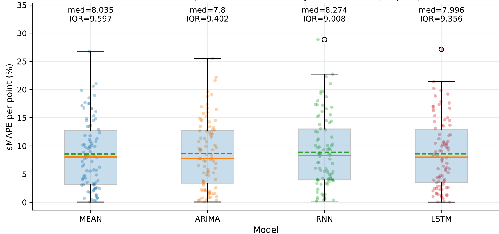
M6_YHUR_SLUR | sMAPE distribution by model — Yd (step=1)
