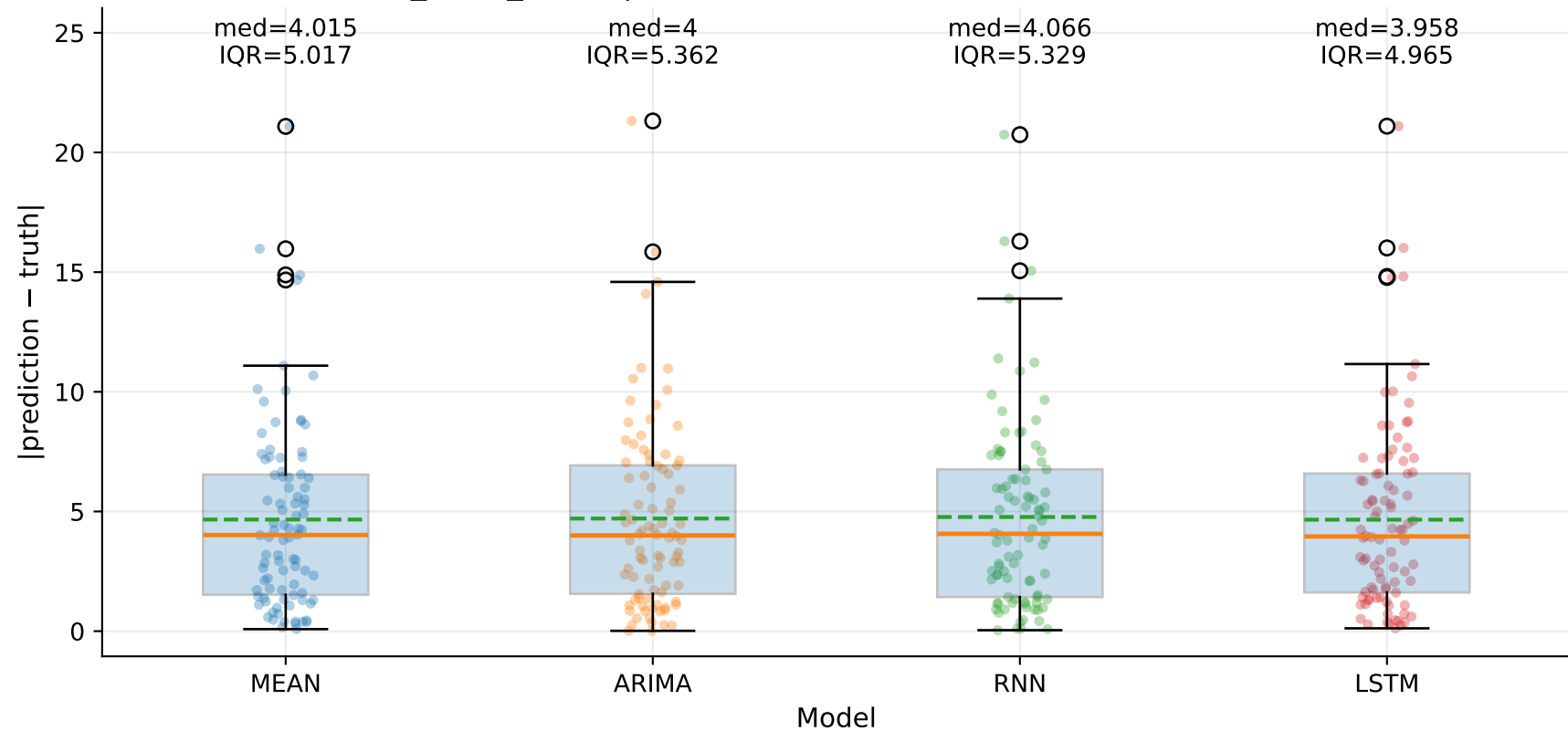
M6_YLUR_SHUR | Absolute error by model — TSEC (step=1)
