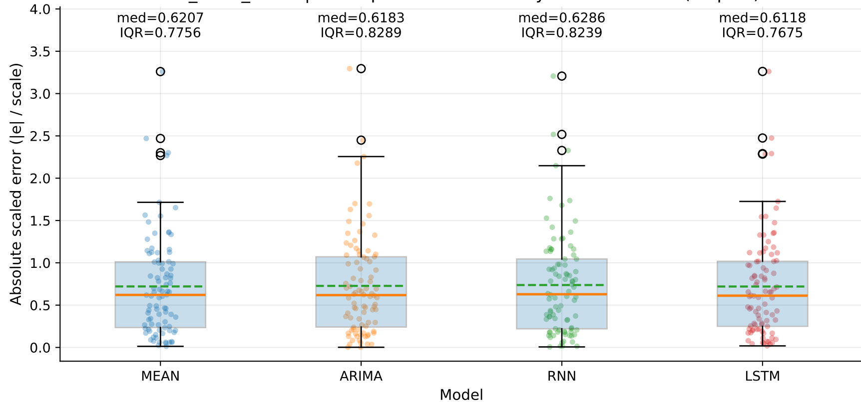
M6_YLUR_SHUR | MASE-point distribution by model — TSEC (step=1)
