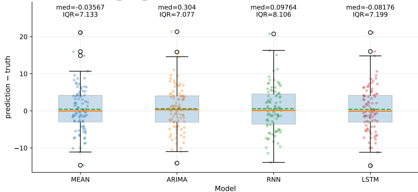
M6_YLUR_SHUR | Signed error by model — TSEC (step=1)
