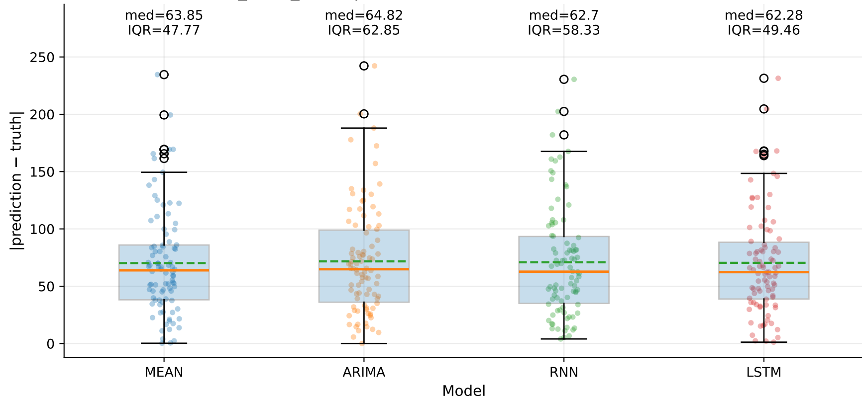
M6_YLUR_SHUR | Absolute error by model — TSE (step=1)
