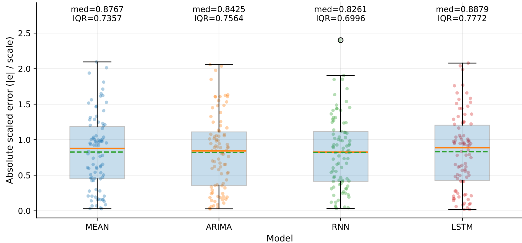
M6_YLUR_SHUR | MASE-point distribution by model — Yd (step=1)
