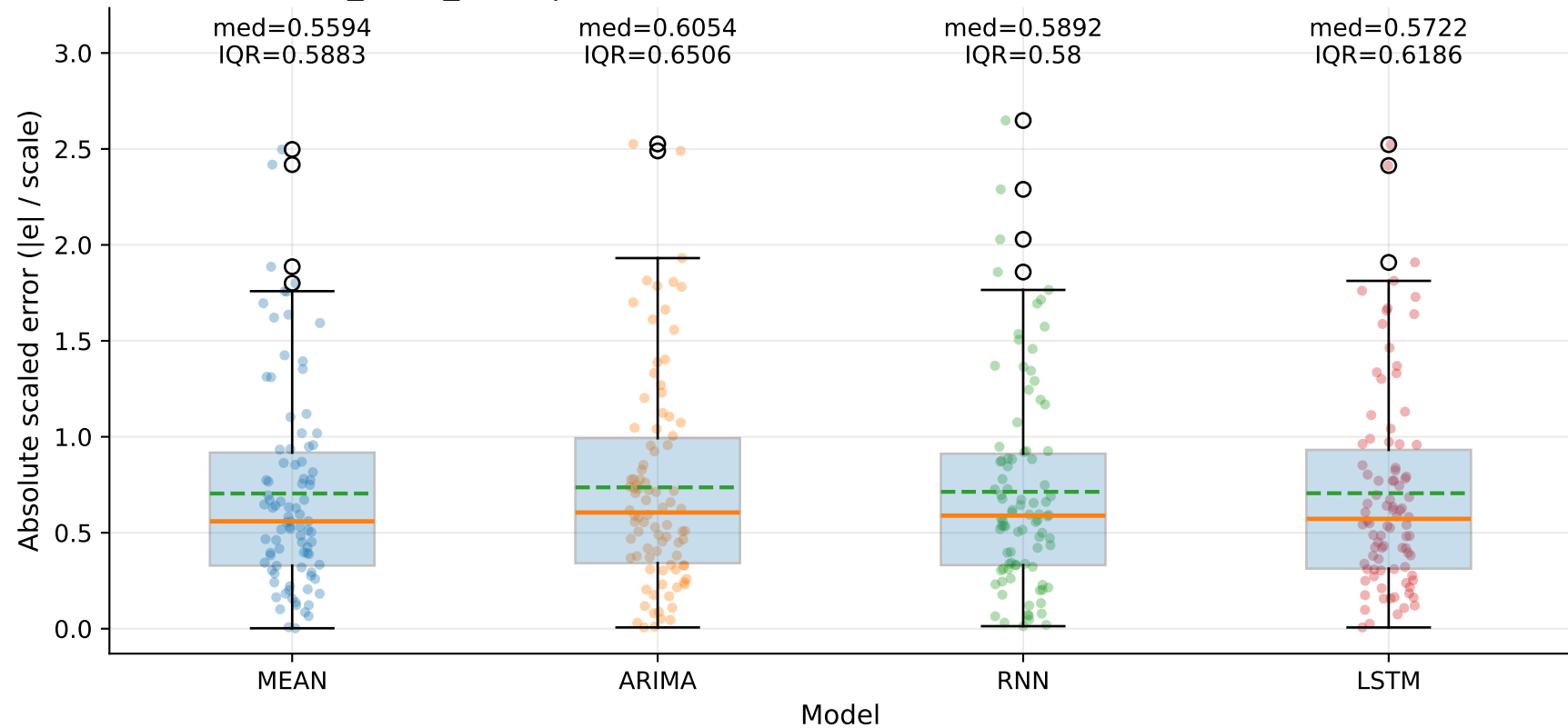
M6_YLUR_SLUR | MASE-point distribution by model — TSEC (step=1)
