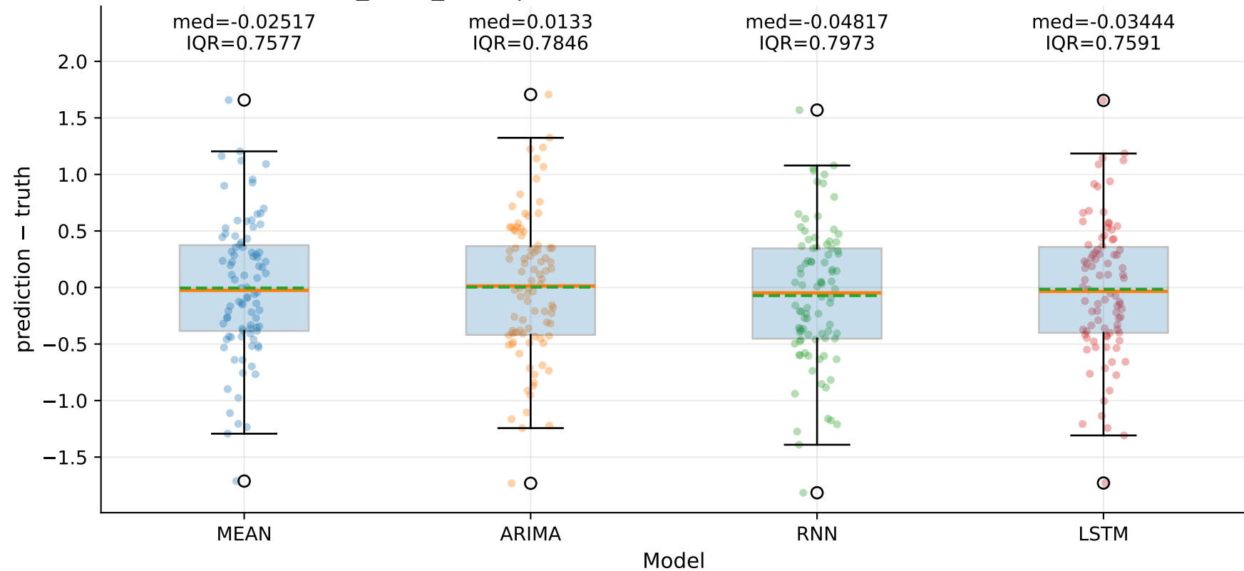
M6_YLUR_SLUR | Signed error by model — TSEC (step=1)
