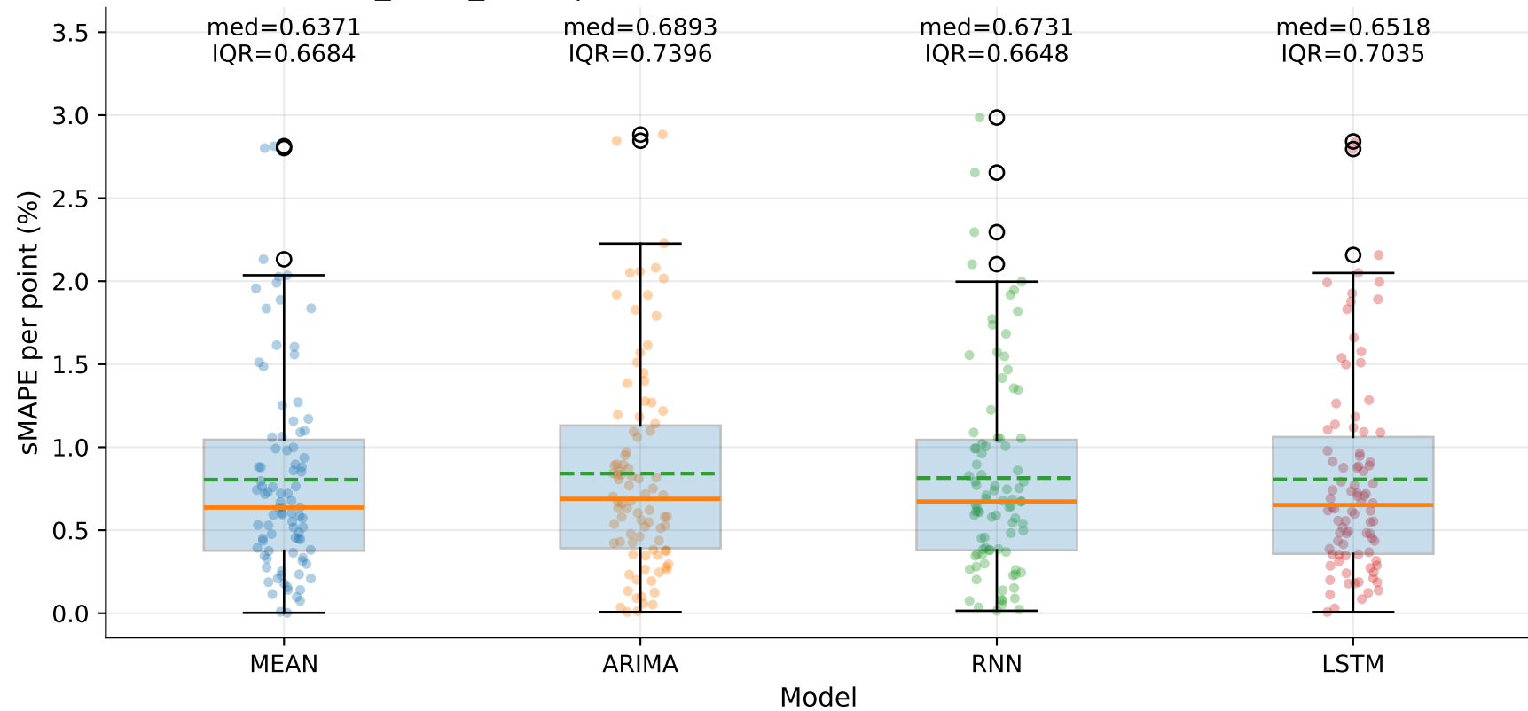
M6_YLUR_SLUR | sMAPE distribution by model — TSEC (step=1)
