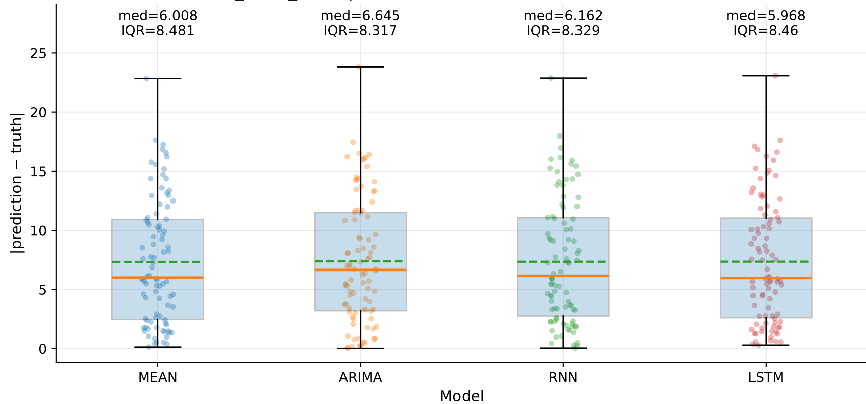
M6_YLUR_SLUR | Absolute error by model — TSE (step=1)
