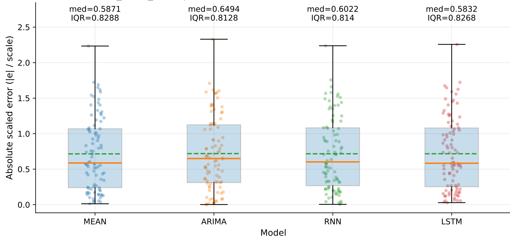
M6_YLUR_SLUR | MASE-point distribution by model — TSE (step=1)
