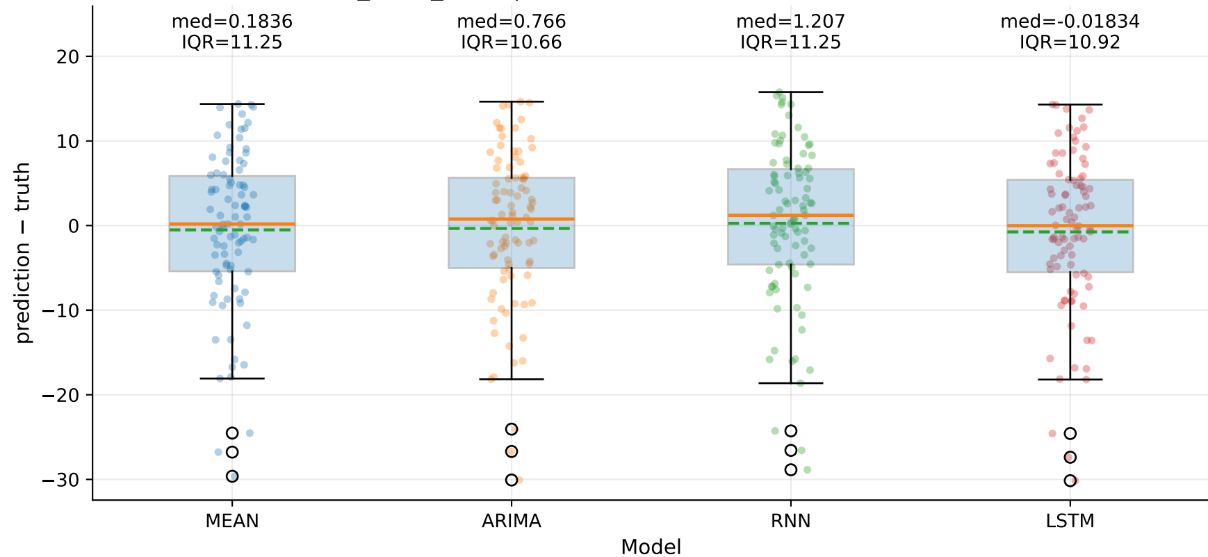
M6_YLUR_SLUR | Signed error by model — Yd (step=1)
