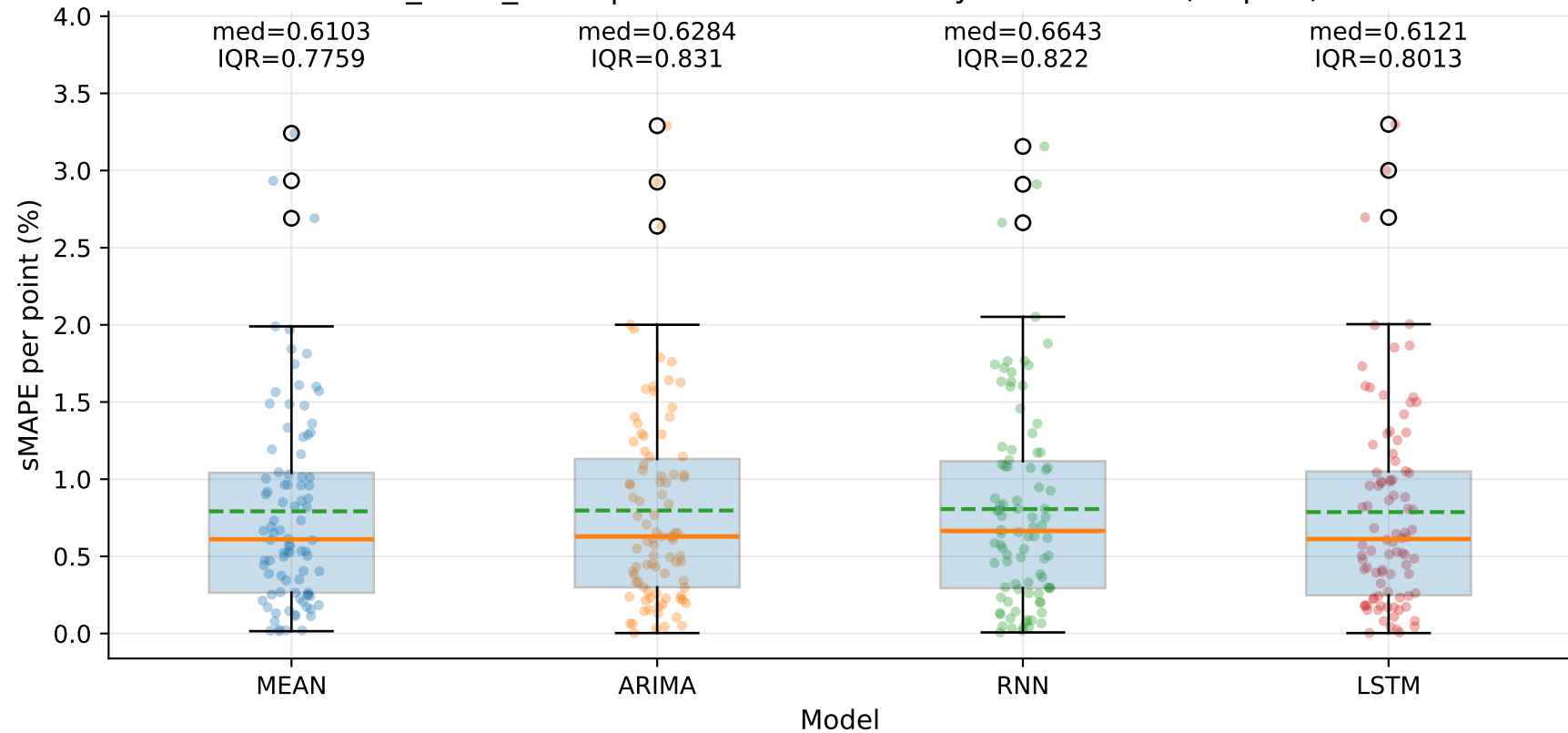
M6_YLUR_SLUR | sMAPE distribution by model — Yd (step=1)
