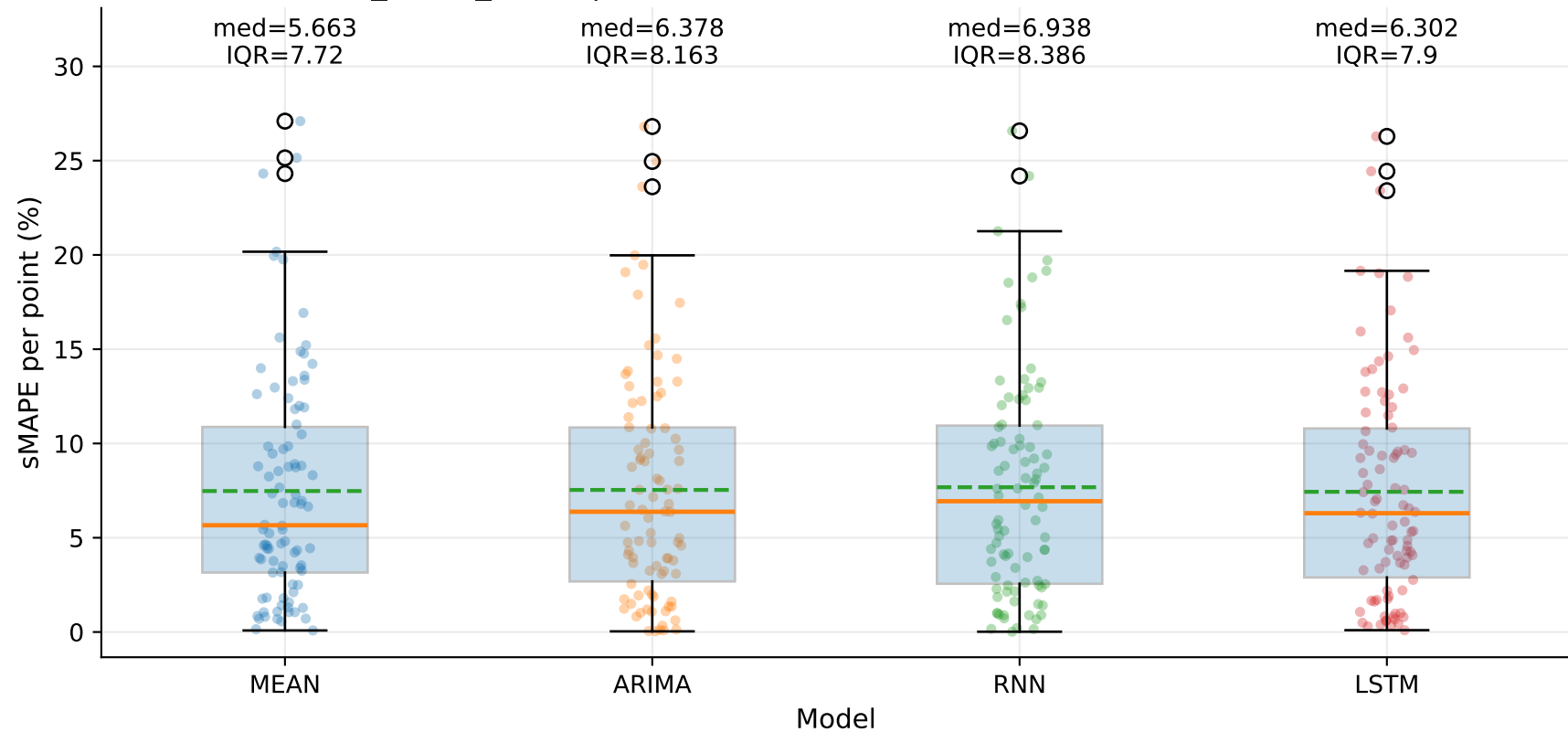
M7_YHUR_SHUR | sMAPE distribution by model — TSEC (step=1)
