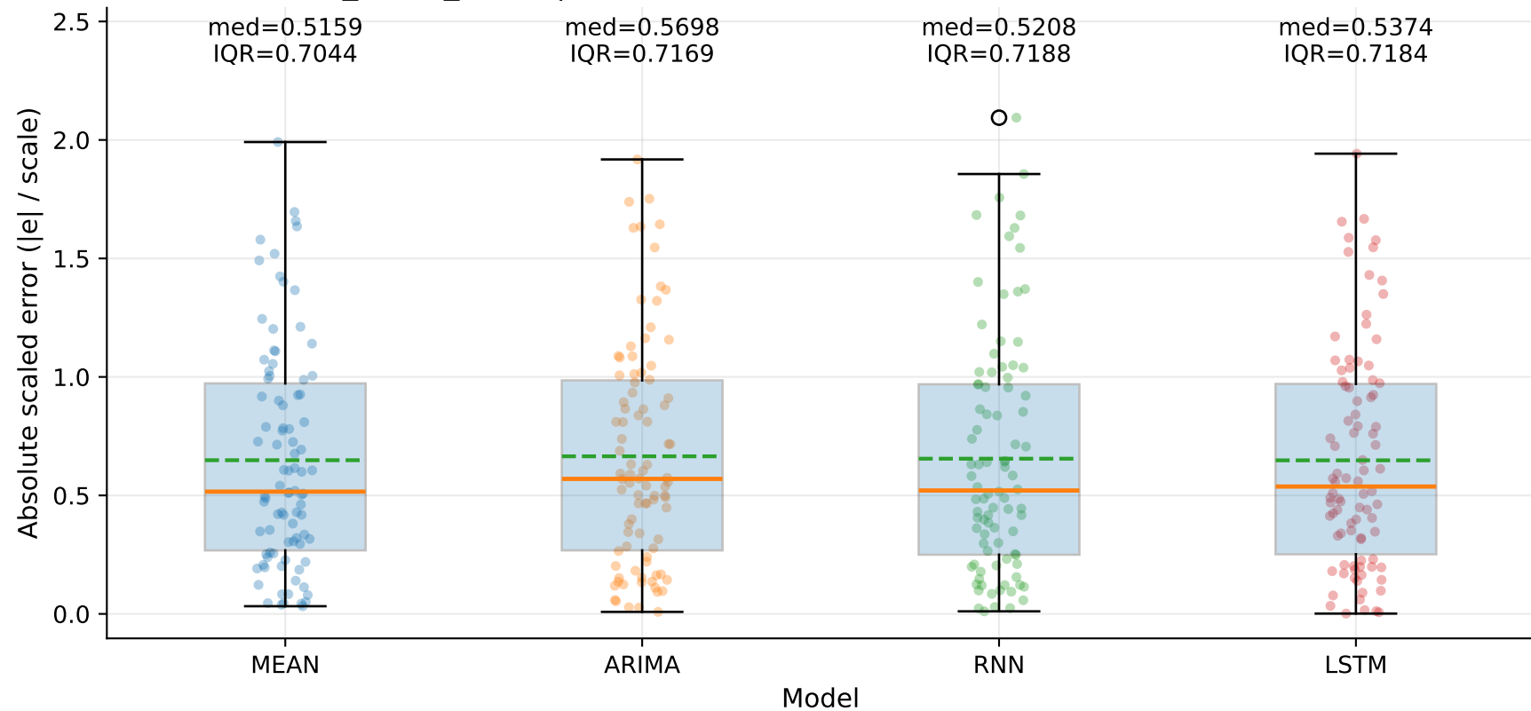
M7_YHUR_SHUR | MASE-point distribution by model — TSE (step=1)
