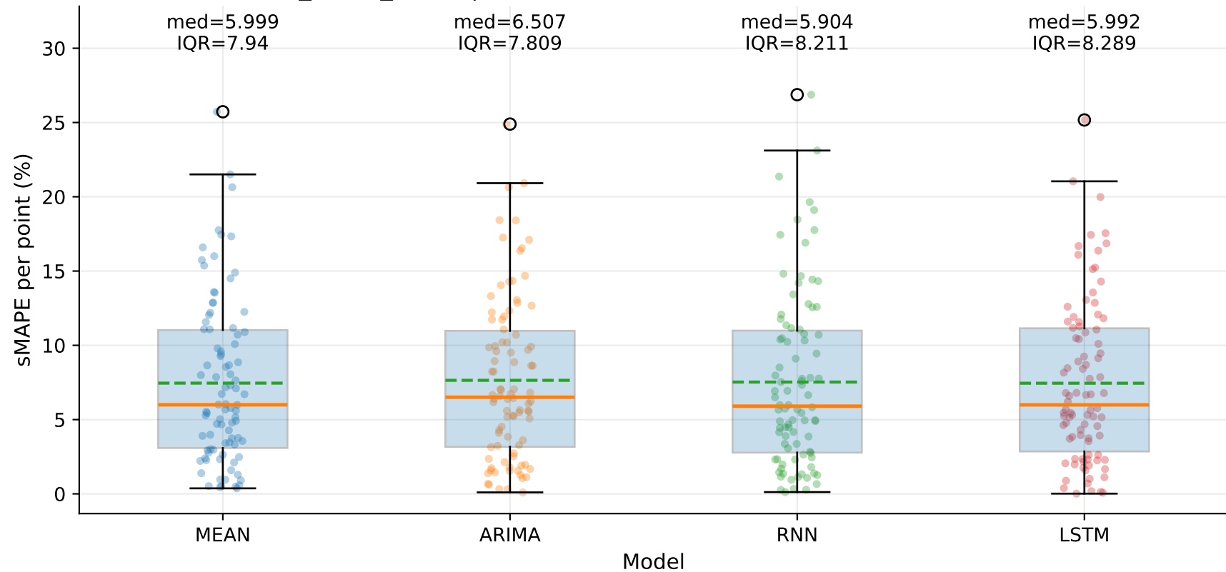
M7_YHUR_SHUR | sMAPE distribution by model — TSE (step=1)
