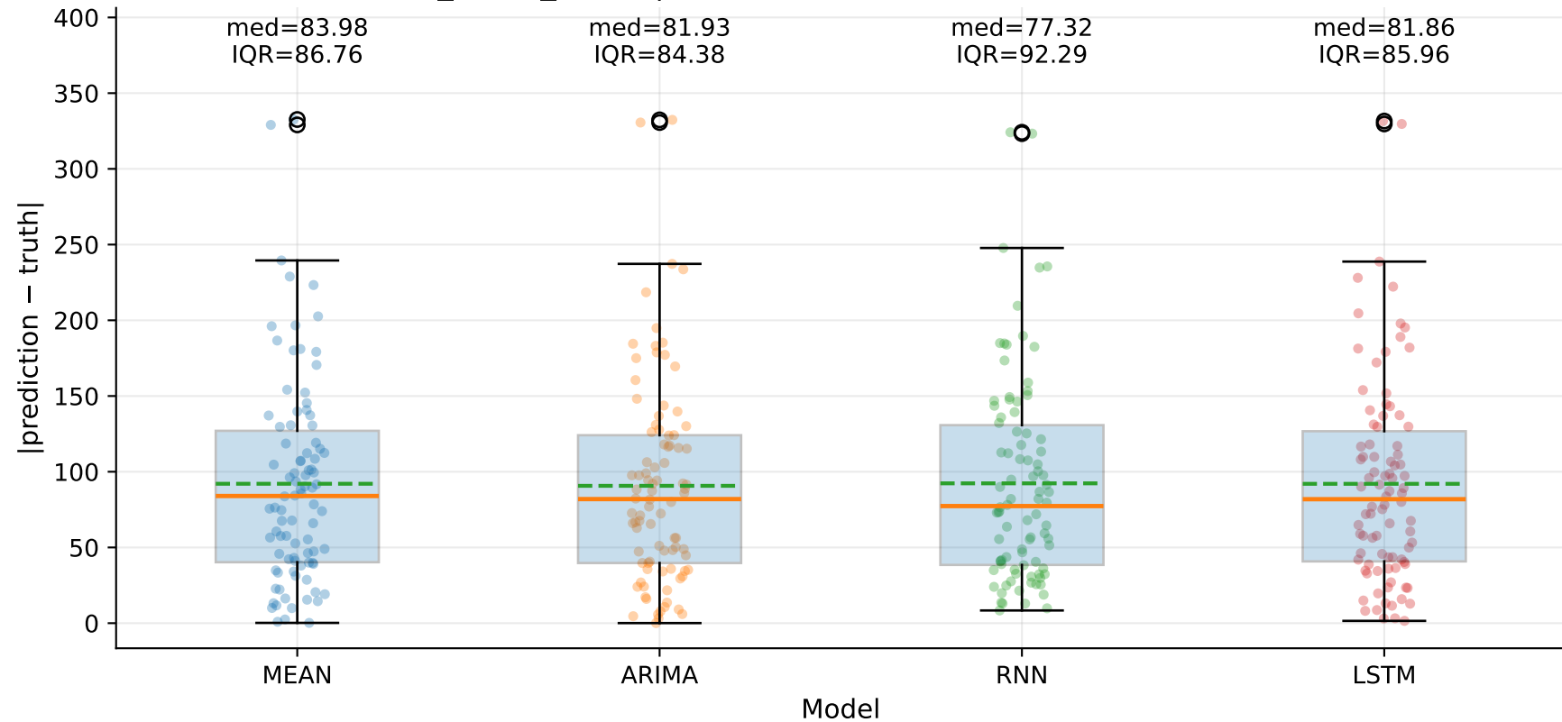
M7_YHUR_SHUR | Absolute error by model — Yd (step=1)
