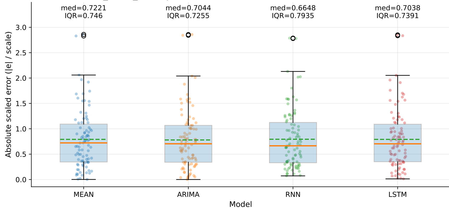
M7_YHUR_SHUR | MASE-point distribution by model — Yd (step=1)
