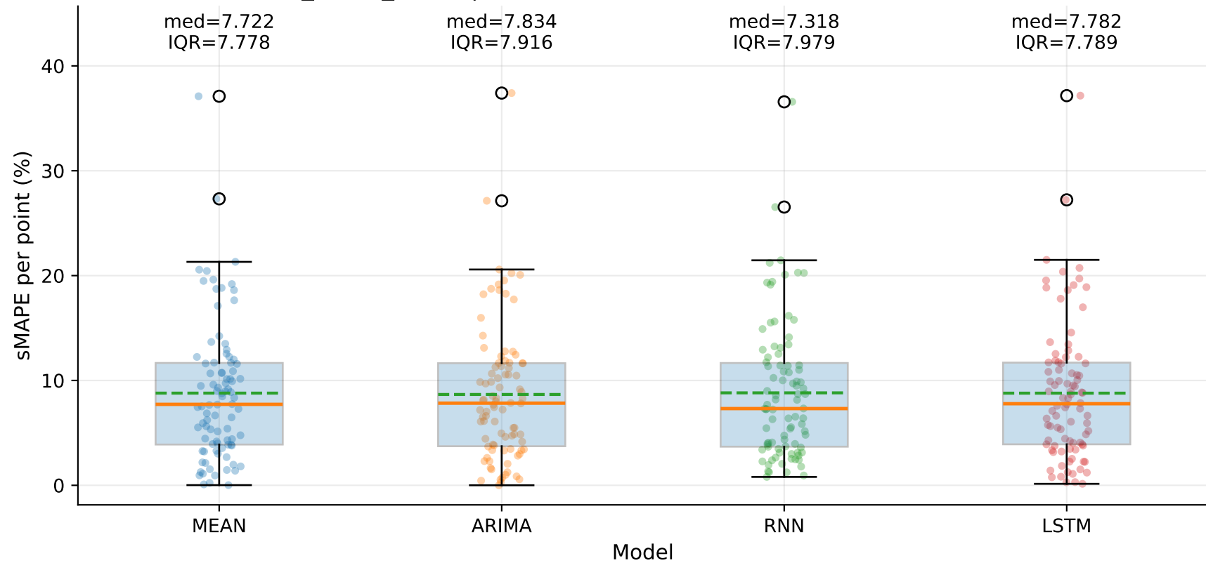
M7_YHUR_SHUR | sMAPE distribution by model — Yd (step=1)
