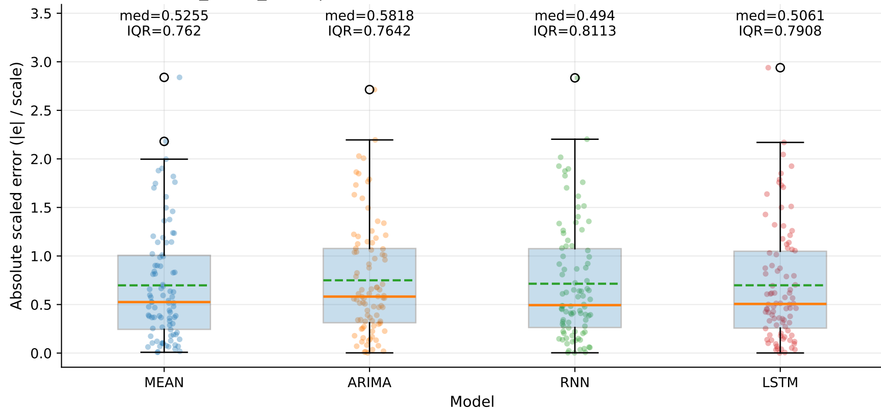
M7_YHUR_SLUR | MASE-point distribution by model — TSE (step=1)
